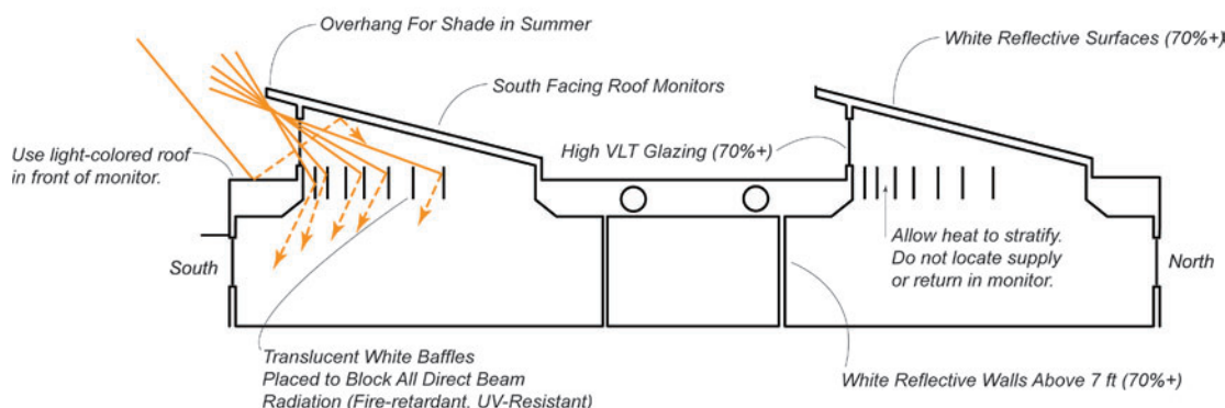
Figure 5.12. Classroom toplighting.
