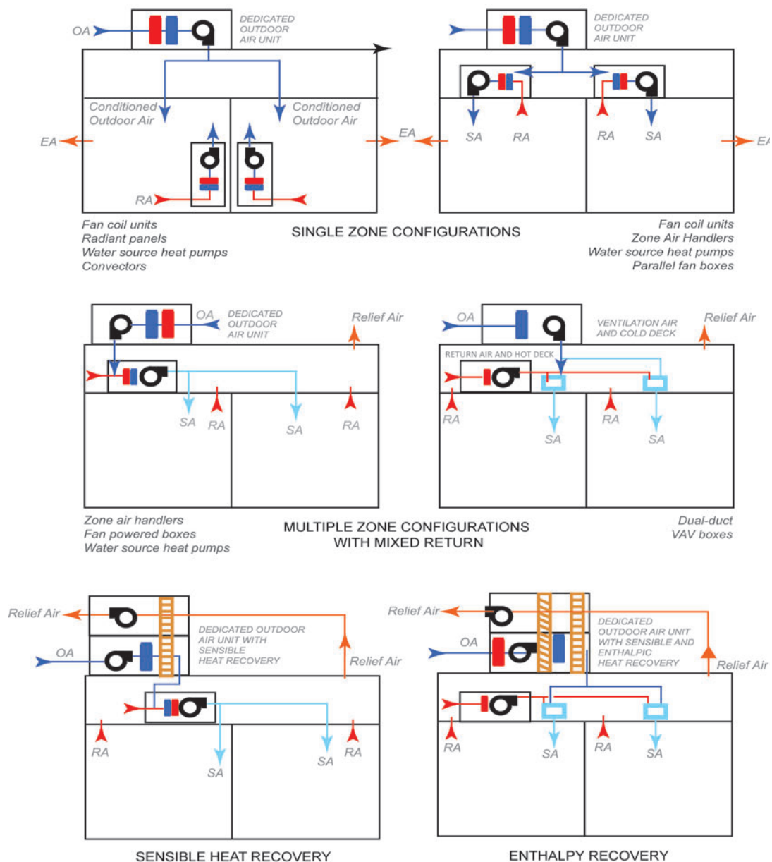
Figure 5.18. Examples of DOAS configurations.
