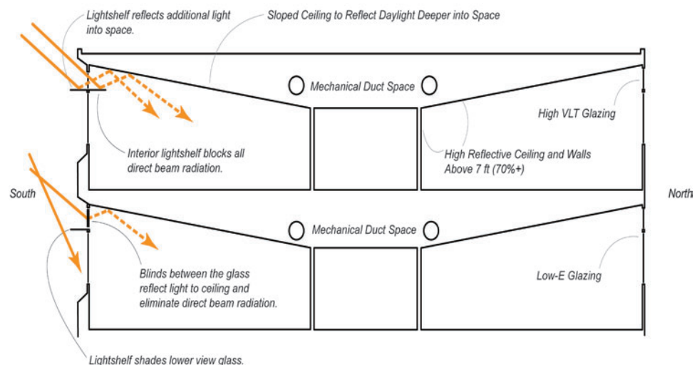
Figure 5.8. Classroom sidelighting.
