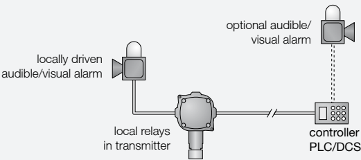
LOCALLY DRIVEN ALARM SYSTEM
